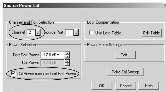
Figure 13. A source power calibration adjusts the output power of the network analyzer for absolute power accuracy.
